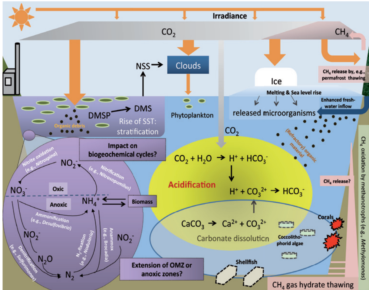
Figure 2.13. Scheme illustrating the potential global change effects on the ocean. Globally increasing temperatures and concentrations of greenhouse gases such as CO 2 and CH 4 will have significant impacts on microbial activities and communities, which may affect biogeochemical cycles. (Developed by Matthias Labrenz)
